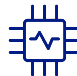
AI/ML Platform
